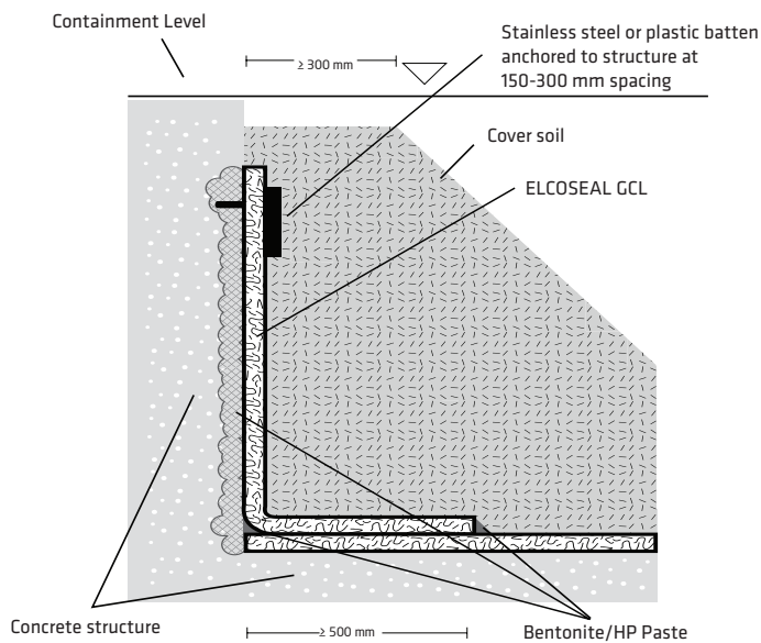
Figure 12b Typical connection to a concrete structure where the Elcoseal panel is required to extend below the maximum containment level
