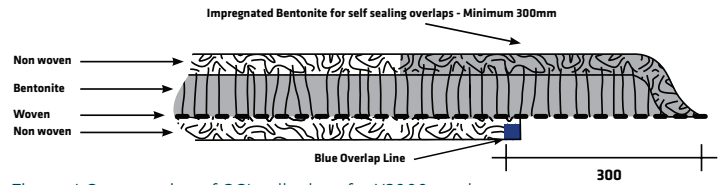
Figure 4 Cross section of GCL roll edges for X2000 grade
