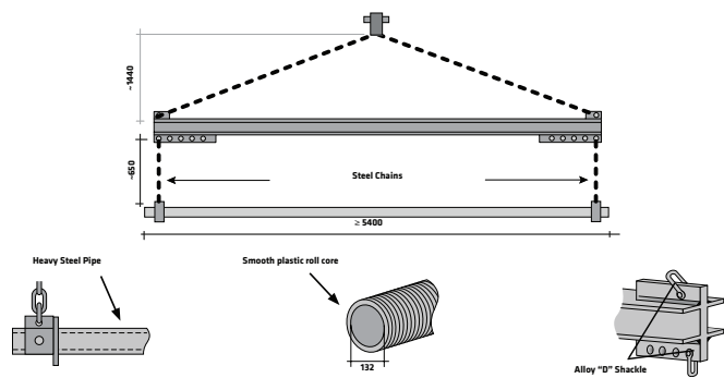
Figure 2 Elcoseal typical Spreader Bar assembly
