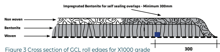
Figure 3 Cross section of GCL roll edges for X1000 grade
