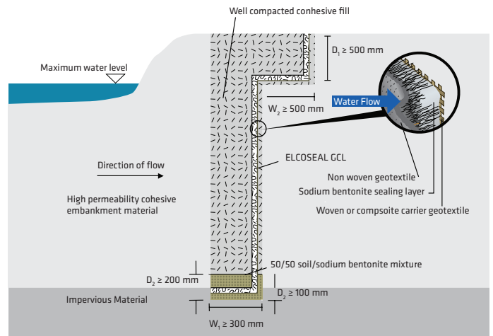
Figure 11 Elcoseal cut off trench detail for cohesive soils
