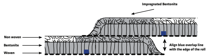
Figure 5 Longitudinal (or edge) overlap with self-sealing impregnated bentonite (X1000 shown)
