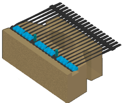
KEYSTONE TW3 POSITIVE CONNECTION MODULAR BLOCK SYSTEM
