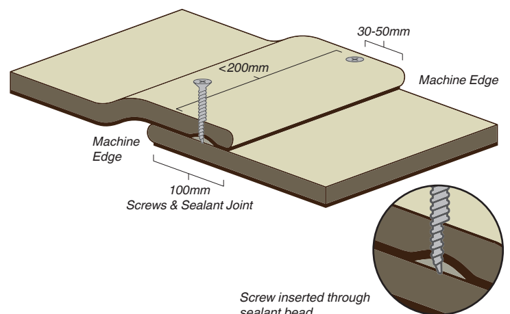
Diagram showing screw inserted through sealant bead
